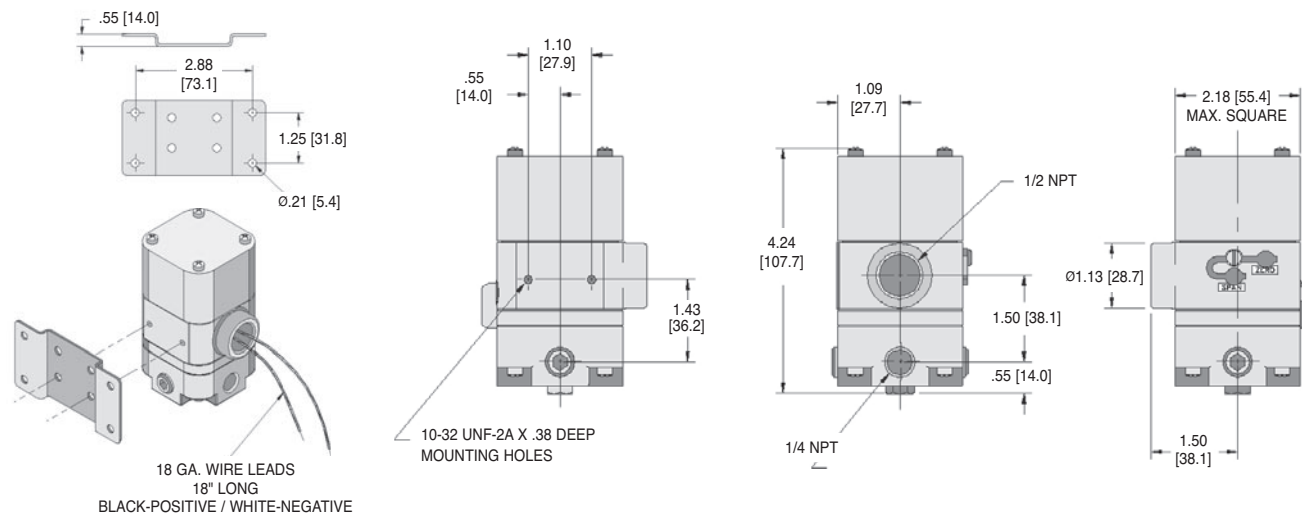
MOUNTING BRACKET
