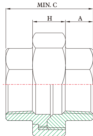
Thread End
