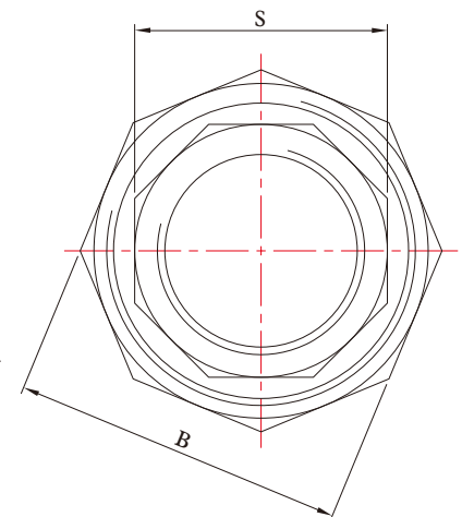
Socket-Weld End
