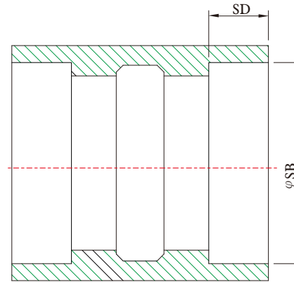
Socket-Weld End
