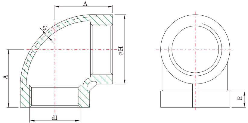
Thread End
