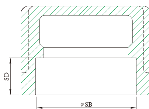
Socket-Weld End
