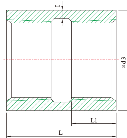
Thread End
