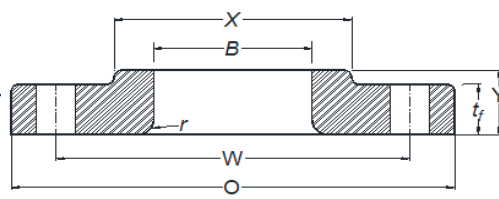
LAPPED FLANGE
