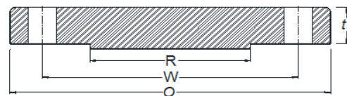
BLIND FLANGE
