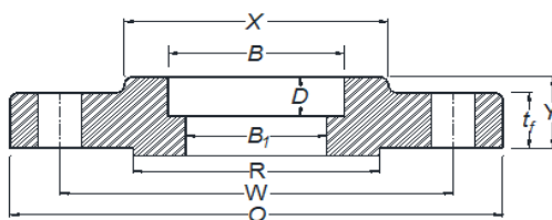
SOCKET WELDING FLANGE
