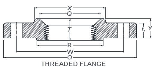
THREADED FLANGE
