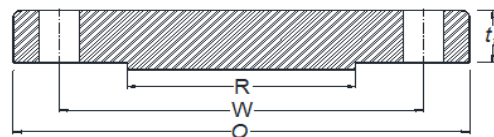
BLIND FLANGE
