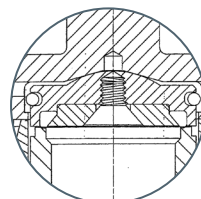
O-RING
